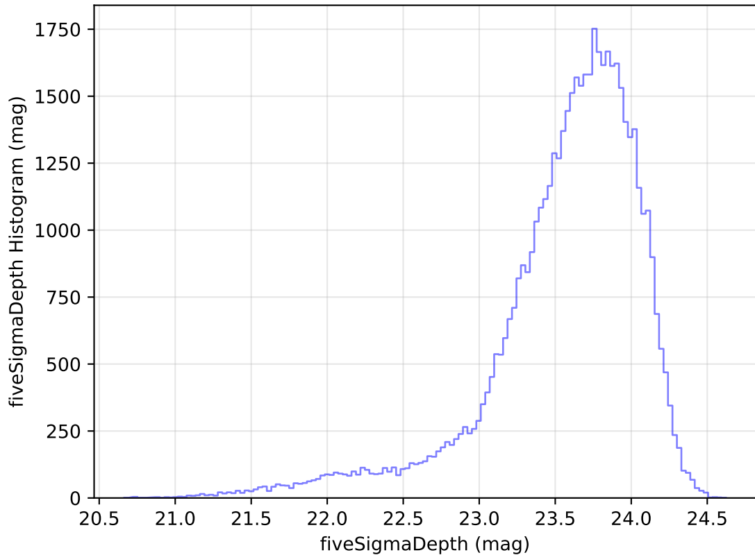
internal_u_expt45_nscale1.1v3.4_10yrs Yr 1 i band: fiveSigmaDepth Histogram
