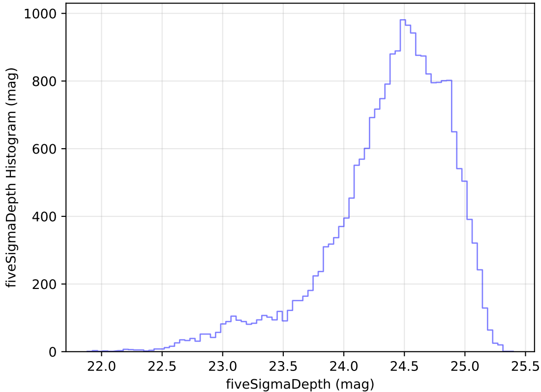
internal_u_expt45_nscale1.1v3.4_10yrs Yr 1 g band: fiveSigmaDepth Histogram
