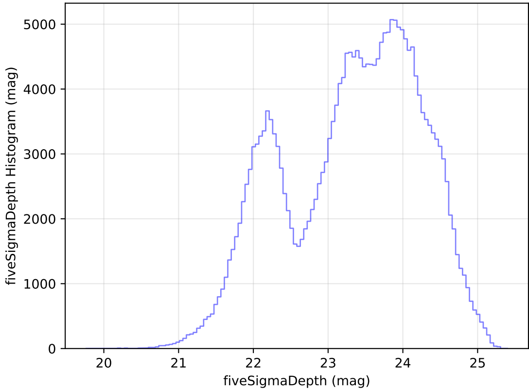
internal_u_expt45_nscale1.1v3.4_10yrs Yr 1 all bands: fiveSigmaDepth Histogram
