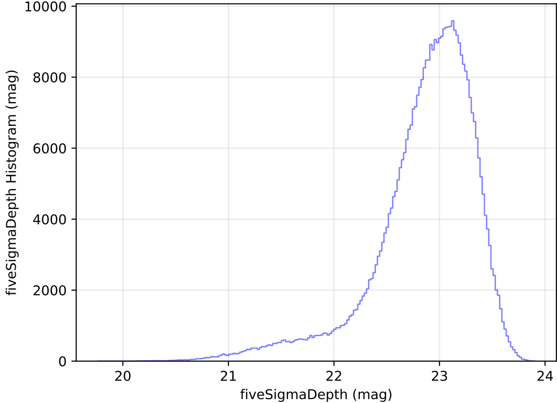
internal_u_expt45_nscale1.1v3.4_10yrs WFD z band: fiveSigmaDepth Histogram
