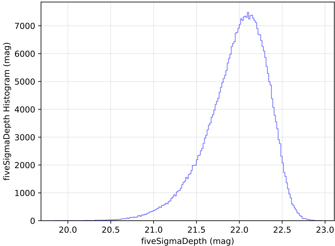
internal_u_expt45_nscale1.1v3.4_10yrs WFD y band: fiveSigmaDepth Histogram
