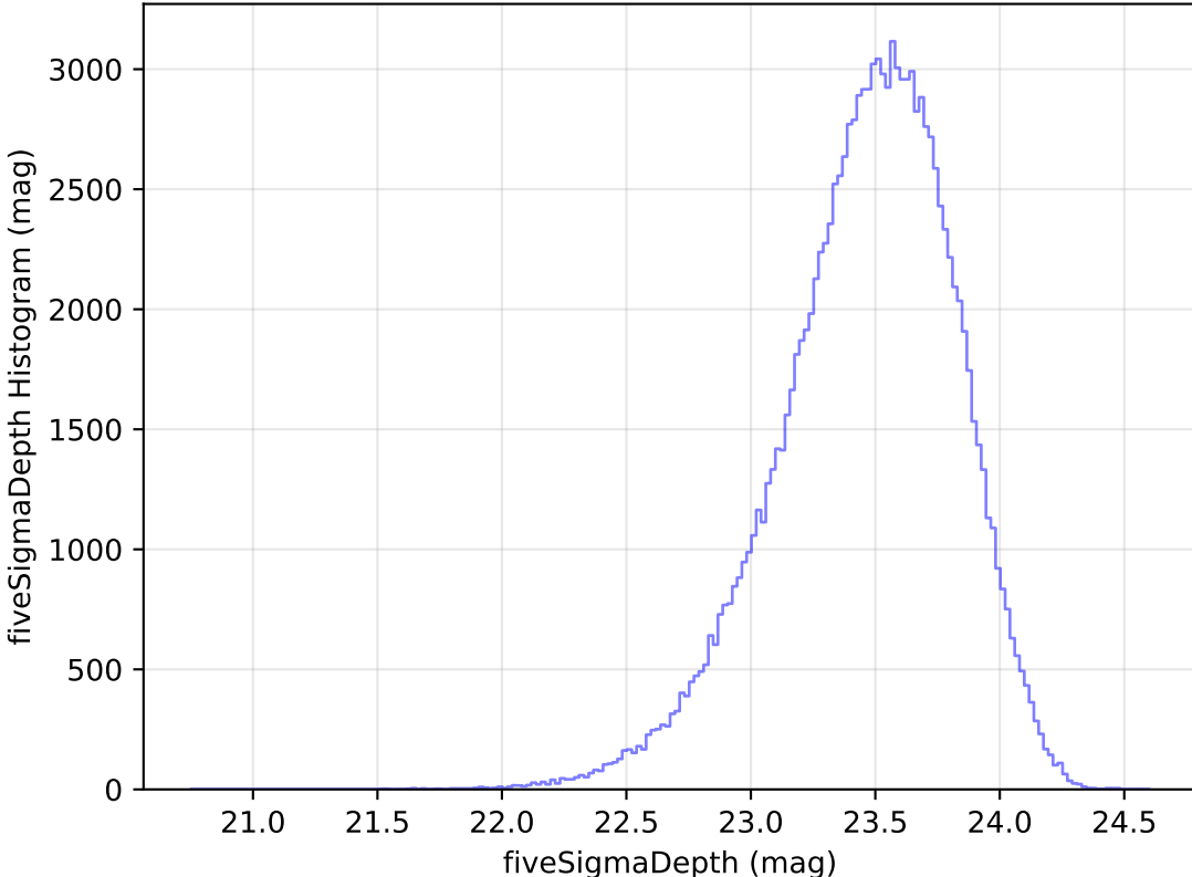
internal_u_expt45_nscale1.1v3.4_10yrs WFD u band: fiveSigmaDepth Histogram
