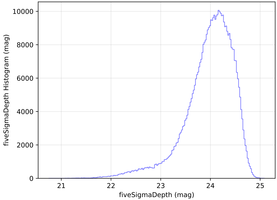
internal_u_expt45_nscale1.1v3.4_10yrs WFD r band: fiveSigmaDepth Histogram
