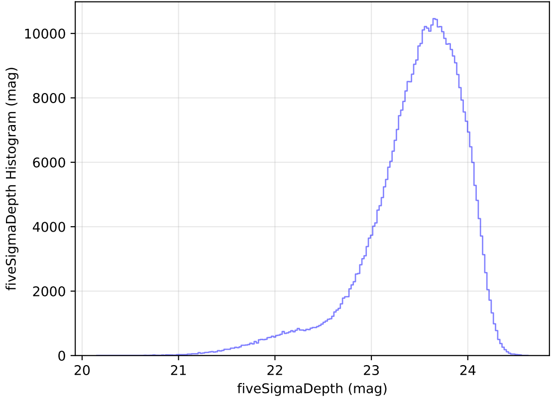
internal_u_expt45_nscale1.1v3.4_10yrs WFD i band: fiveSigmaDepth Histogram
