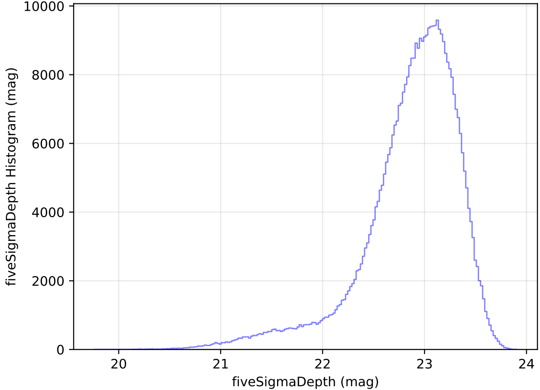
internal_u_expt45_nscale1.1v3.4_10yrs All sky z band: fiveSigmaDepth Histogram
