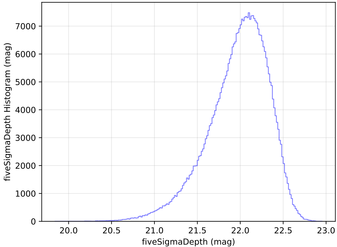
internal_u_expt45_nscale1.1v3.4_10yrs All sky y band: fiveSigmaDepth Histogram
