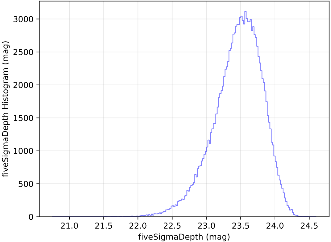
internal_u_expt45_nscale1.1v3.4_10yrs All sky u band: fiveSigmaDepth Histogram
