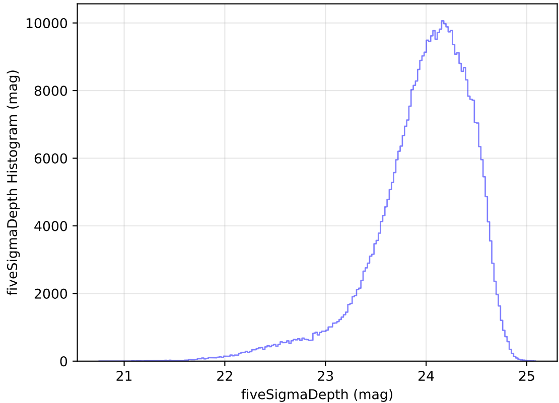
internal_u_expt45_nscale1.1v3.4_10yrs All sky r band: fiveSigmaDepth Histogram
