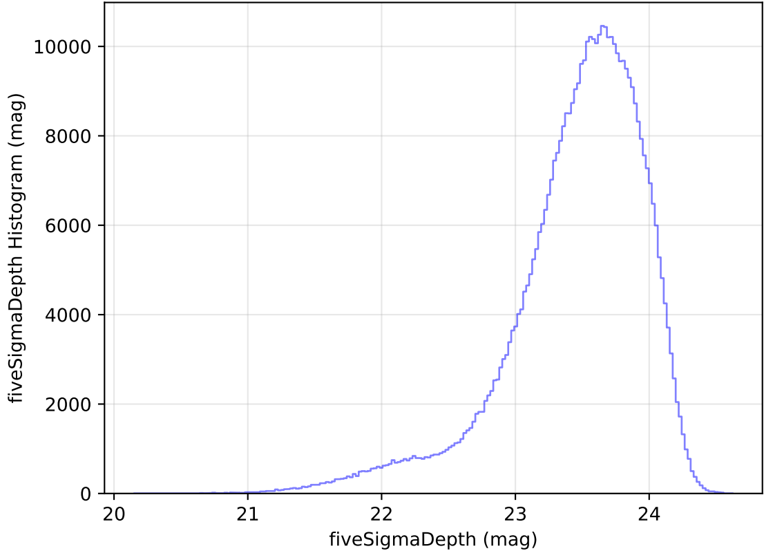
internal_u_expt45_nscale1.1v3.4_10yrs All sky i band: fiveSigmaDepth Histogram
