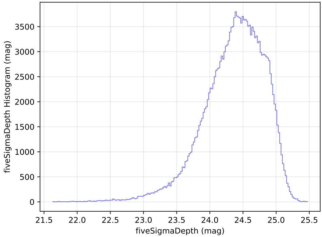
internal_u_expt45_nscale1.1v3.4_10yrs All sky g band: fiveSigmaDepth Histogram
