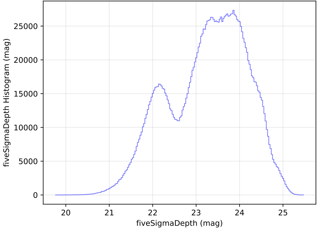
internal_u_expt45_nscale1.1v3.4_10yrs All sky all bands: fiveSigmaDepth Histogram
