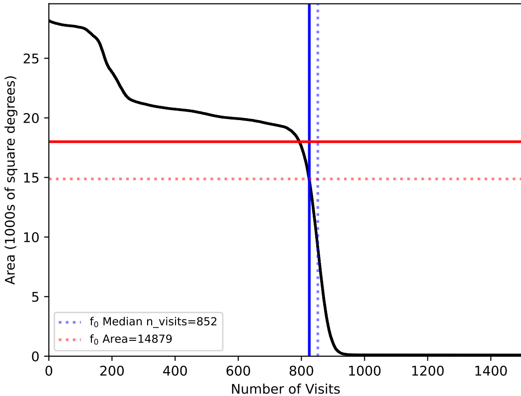
internal_u_expt45_nscale1.1v3.4_10yrs All sky: f0
