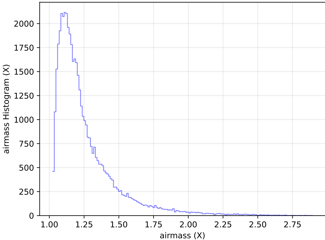
internal_u_expt45_nscale1.1v3.4_10yrs Yr 1 y band: airmass Histogram
