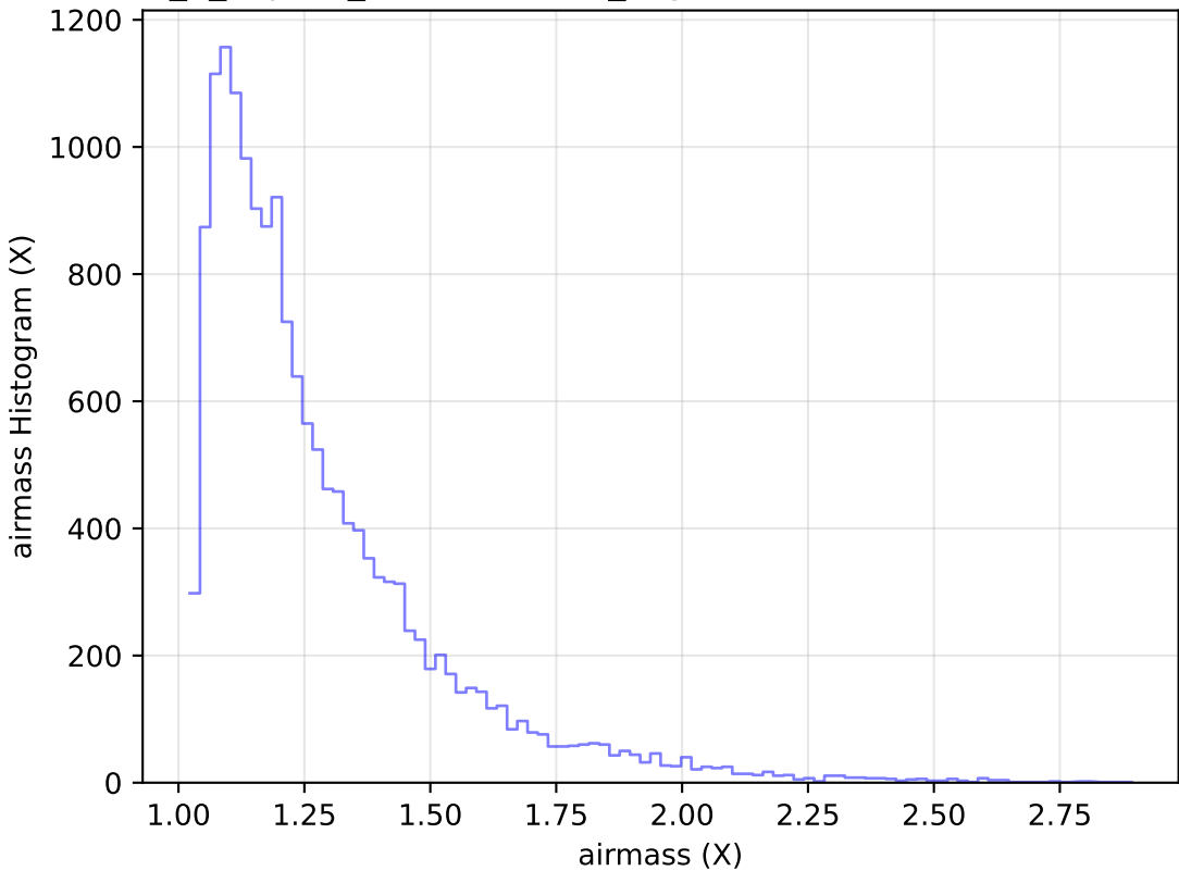
internal_u_expt45_nscale1.1v3.4_10yrs Yr 1 u band: airmass Histogram
