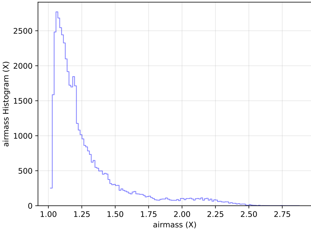
internal_u_expt45_nscale1.1v3.4_10yrs Yr 1 r band: airmass Histogram
