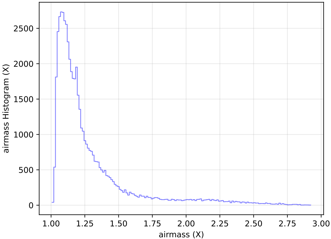
internal_u_expt45_nscale1.1v3.4_10yrs Yr 1 i band: airmass Histogram
