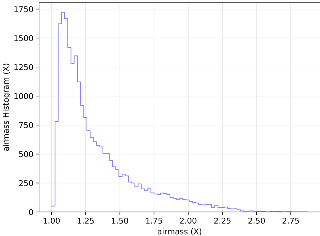
internal_u_expt45_nscale1.1v3.4_10yrs Yr 1 g band: airmass Histogram
