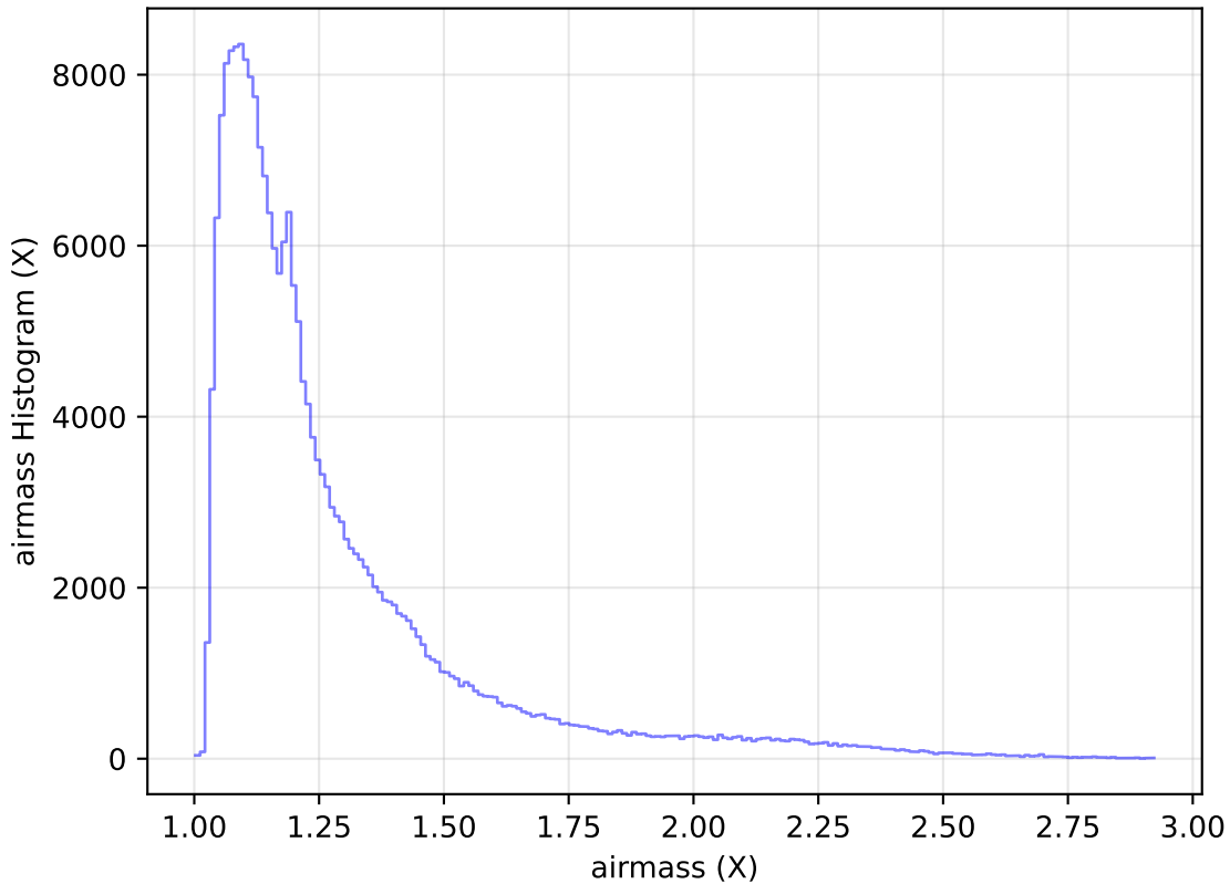
internal_u_expt45_nscale1.1v3.4_10yrs Yr 1 all bands: airmass Histogram
