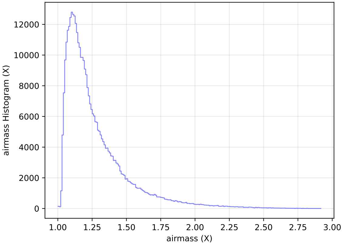
internal_u_expt45_nscale1.1v3.4_10yrs WFD y band: airmass Histogram
