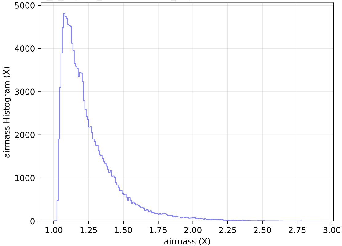
internal_u_expt45_nscale1.1v3.4_10yrs WFD u band: airmass Histogram
