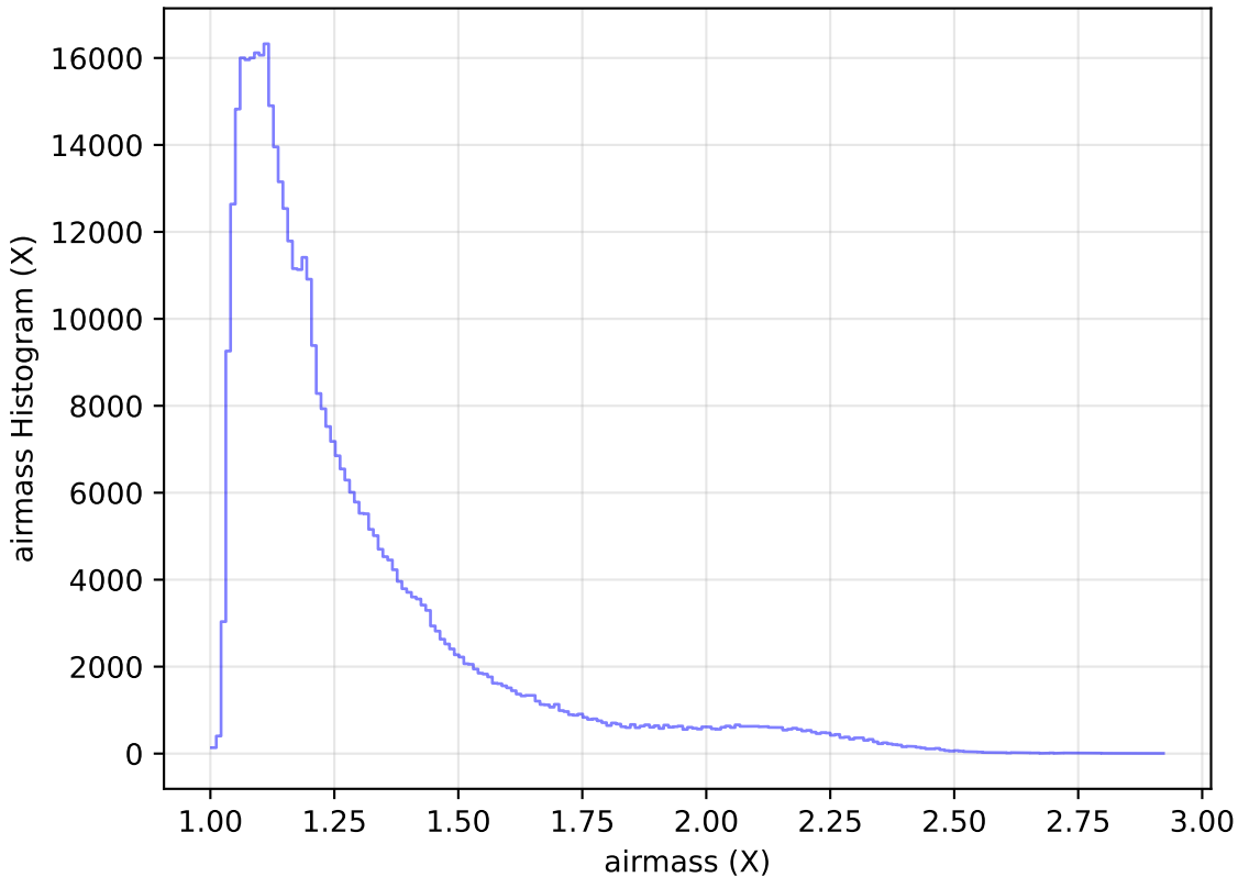
internal_u_expt45_nscale1.1v3.4_10yrs WFD r band: airmass Histogram
