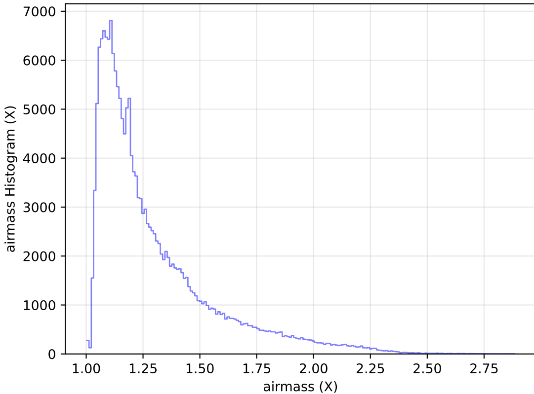
internal_u_expt45_nscale1.1v3.4_10yrs WFD g band: airmass Histogram
