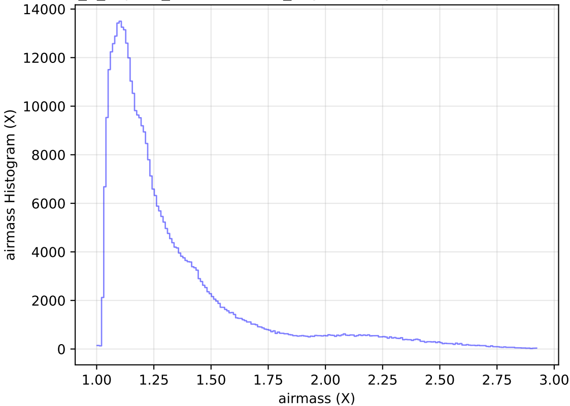
internal_u_expt45_nscale1.1v3.4_10yrs All sky z band: airmass Histogram
