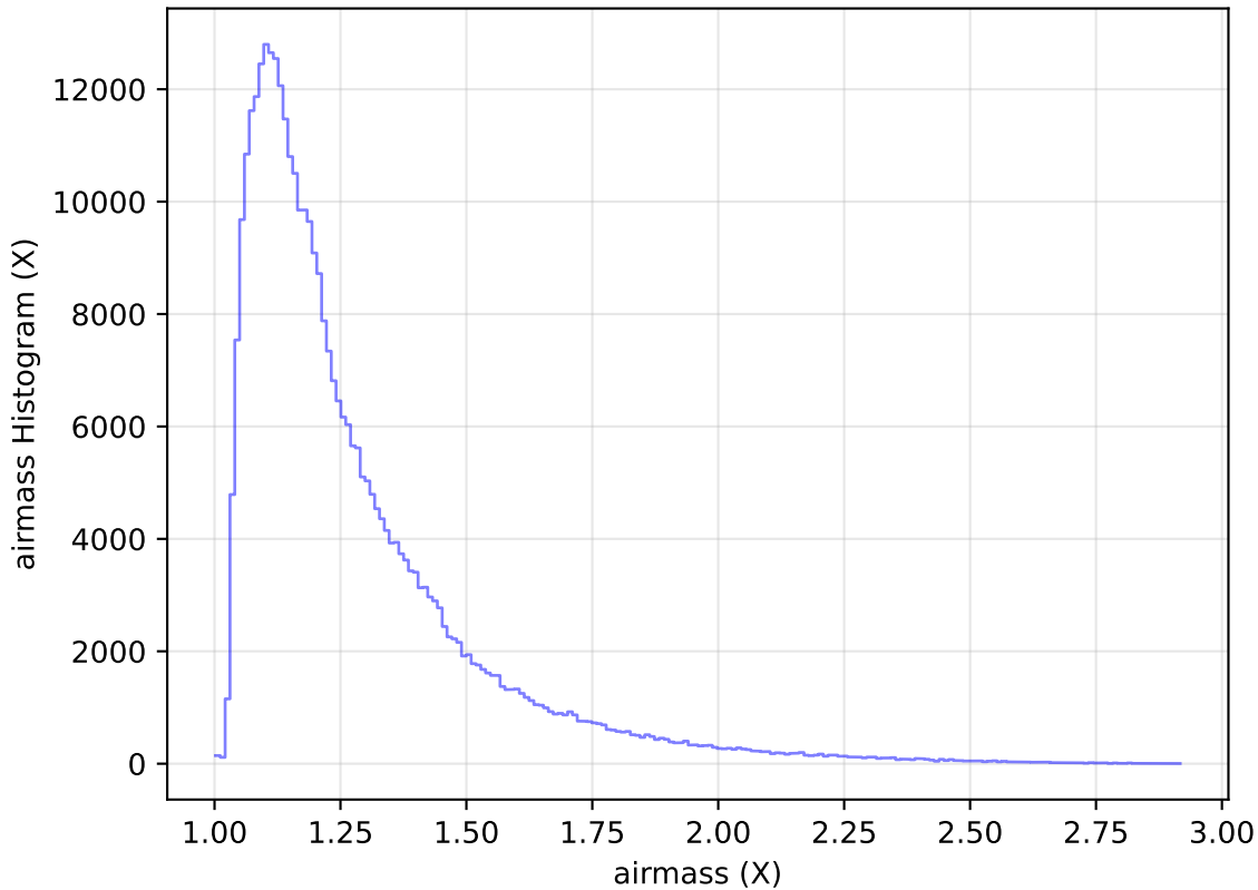
internal_u_expt45_nscale1.1v3.4_10yrs All sky y band: airmass Histogram
