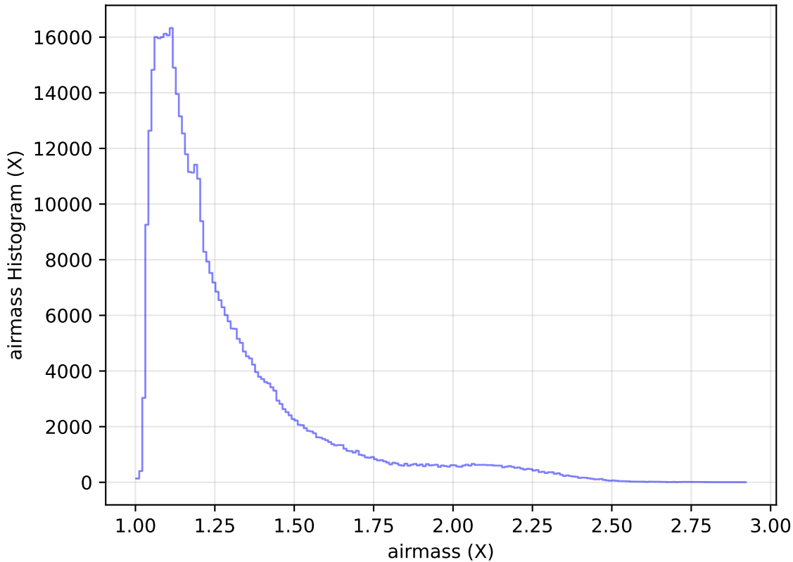
internal_u_expt45_nscale1.1v3.4_10yrs All sky r band: airmass Histogram
