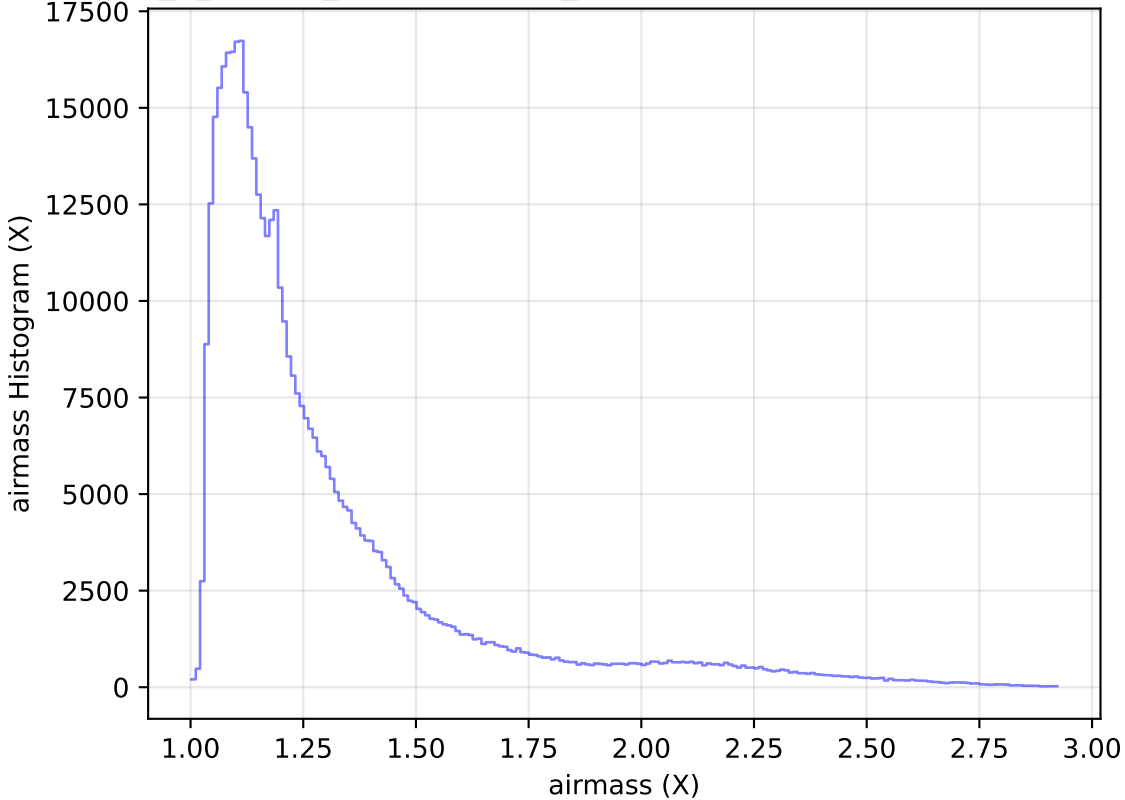
internal_u_expt45_nscale1.1v3.4_10yrs All sky i band: airmass Histogram
