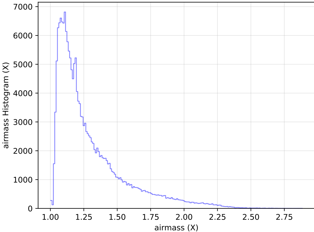
internal_u_expt45_nscale1.1v3.4_10yrs All sky g band: airmass Histogram
