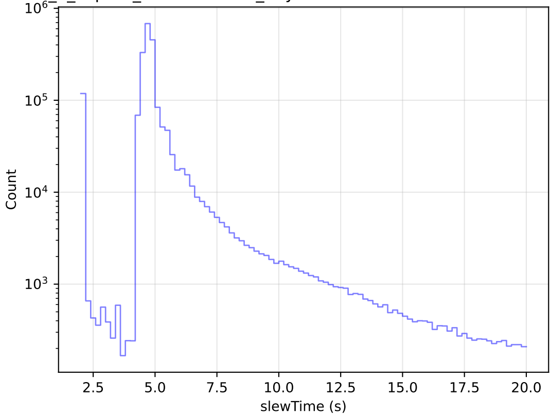
internal_u_expt45_nscale1.1v3.4_10yrs All visits: Zoom Slew Time Histogram
