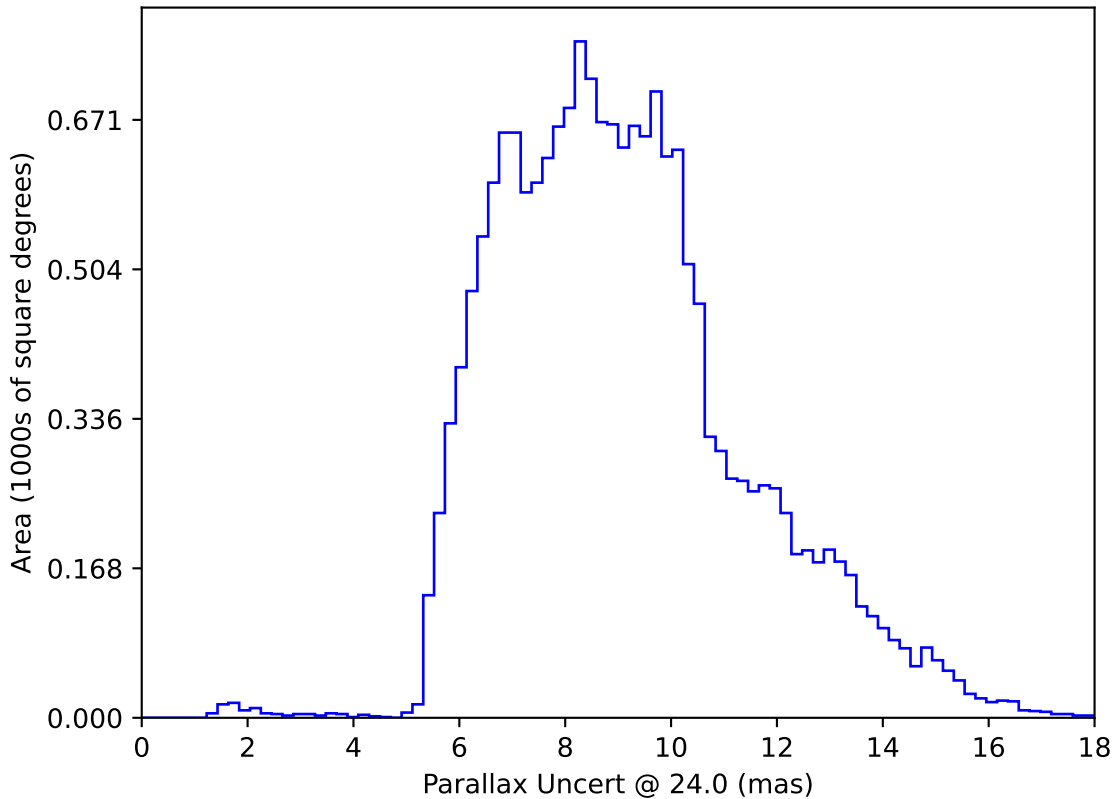
internal_u_expt45_nscale1.1v3.4_10yrs WFD: Parallax Uncert @ 24.0
