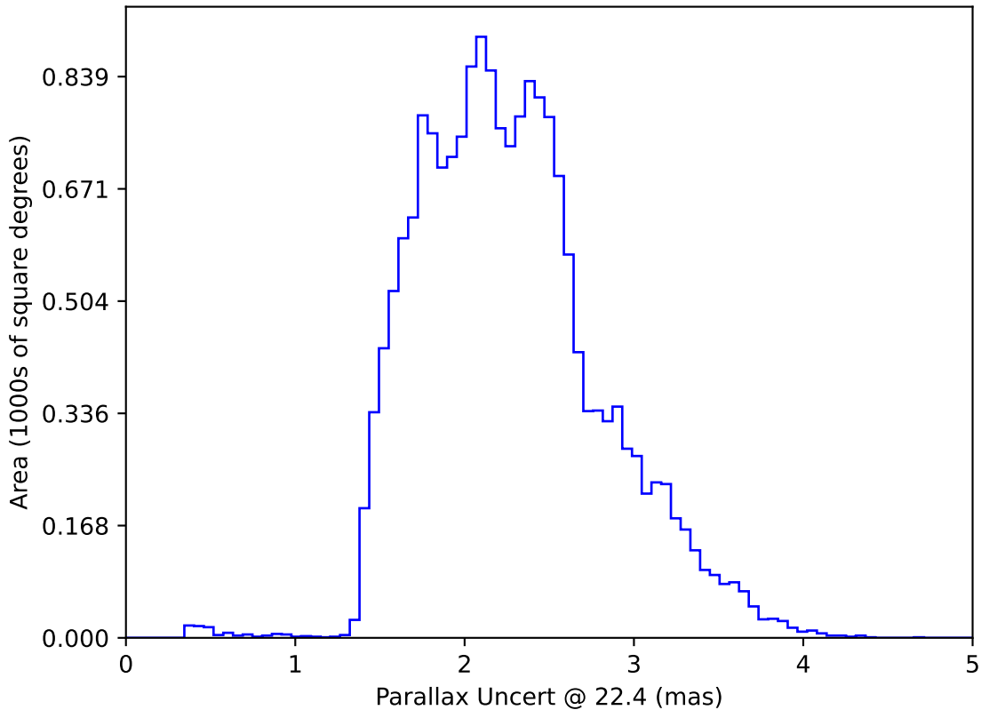
internal_u_expt45_nscale1.1v3.4_10yrs WFD: Parallax Uncert @ 22.4
