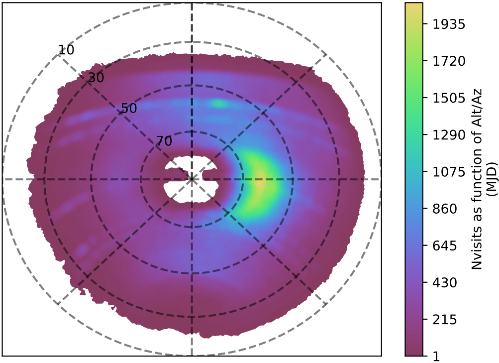
internal_u_expt45_nscale1.1v3.4_10yrs y band: Nvisits as function of Alt/Az
