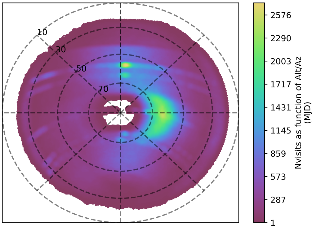
internal_u_expt45_nscale1.1v3.4_10yrs i band: Nvisits as function of Alt/Az
