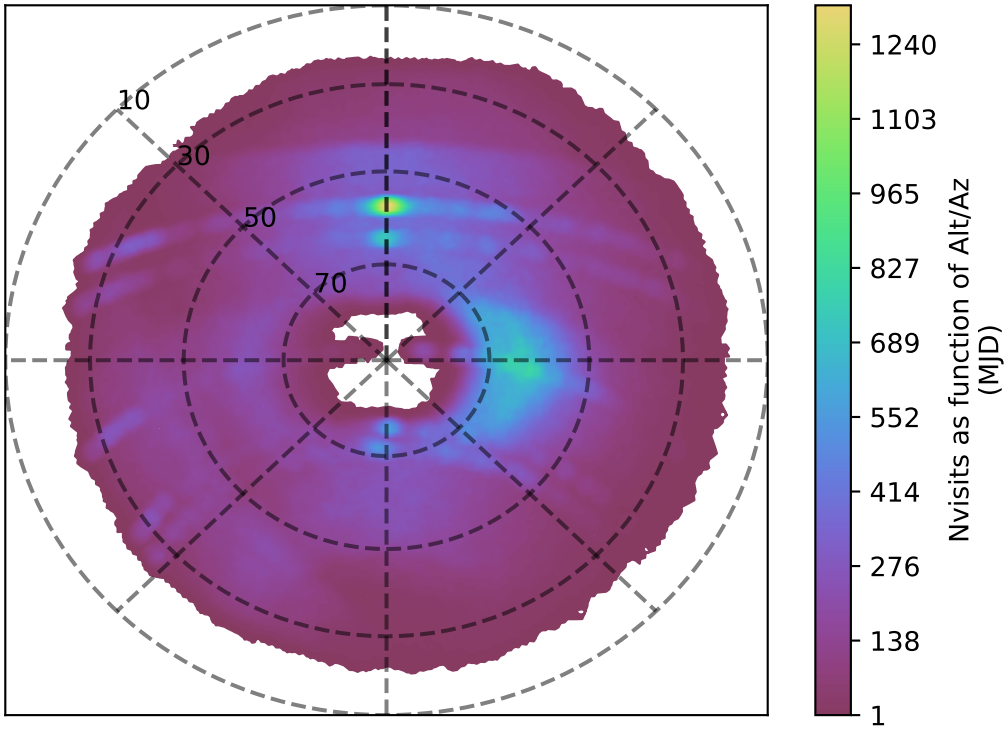
internal_u_expt45_nscale1.1v3.4_10yrs g band: Nvisits as function of Alt/Az
