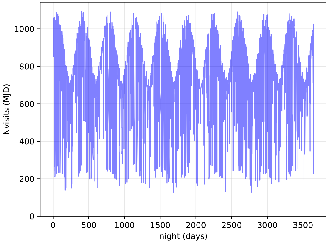
internal_u_expt45_nscale1.1v3.4_10yrs All visits: Nvisits
