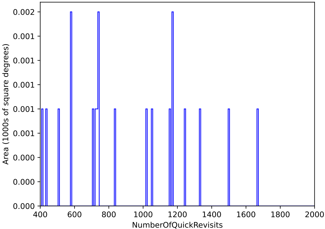
internal_u_expt45_nscale1.1v3.4_10yrs WFD: NumberOfQuickRevisits
