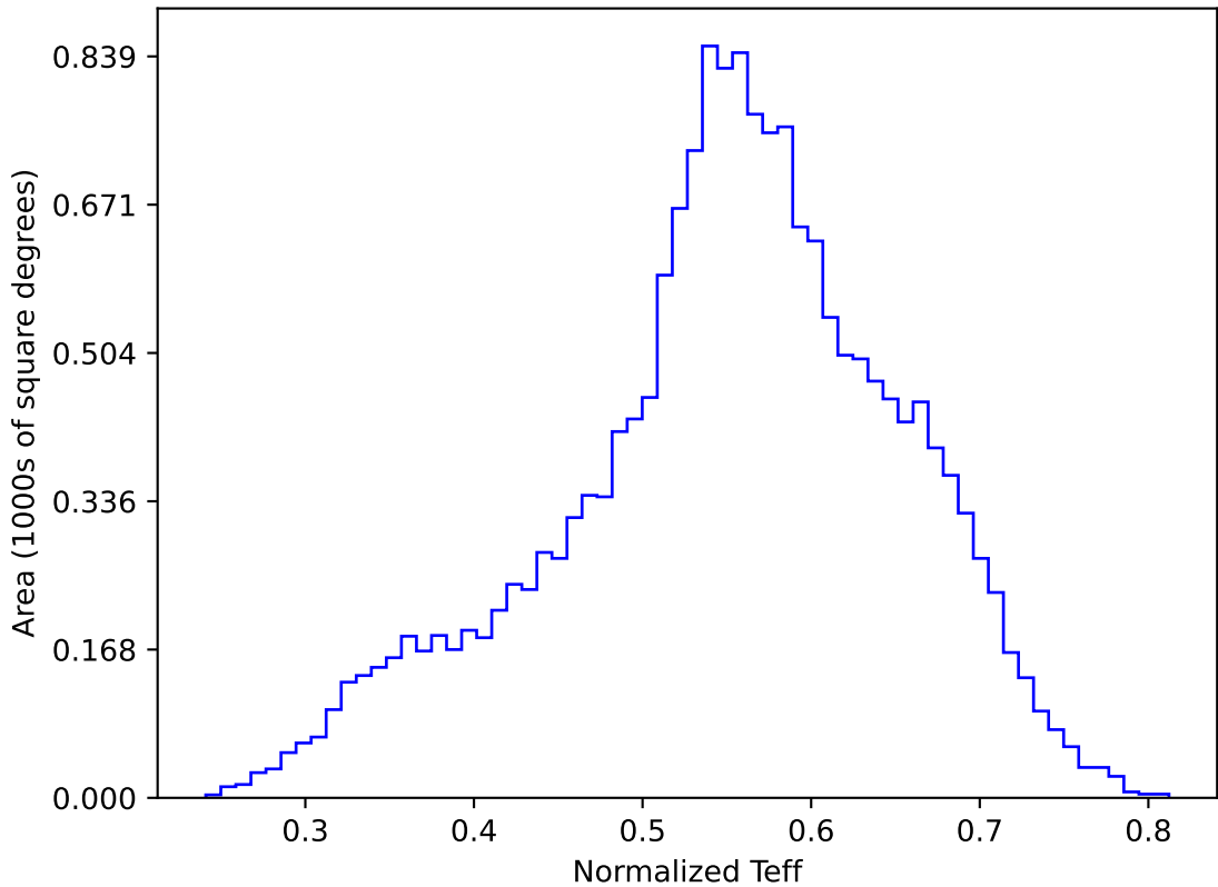
internal_u_expt45_nscale1.1v3.4_10yrs WFD y band: Normalized Teff
