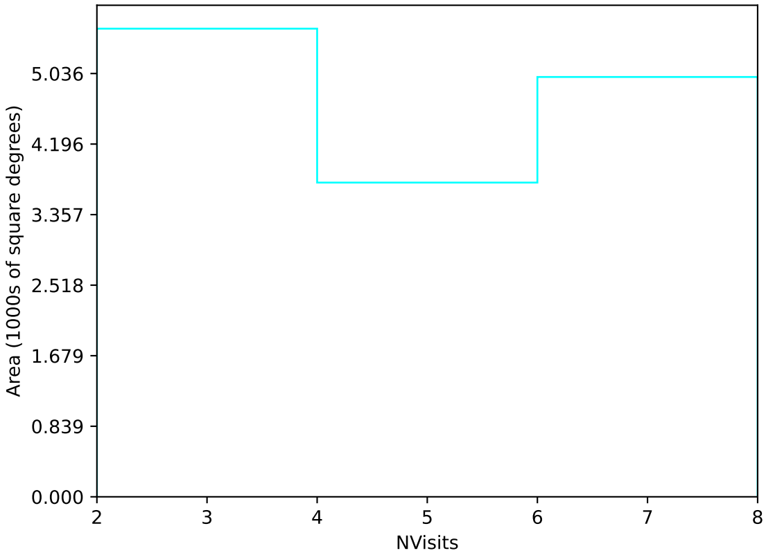
internal_u_expt45_nscale1.1v3.4_10yrs Yr 3-4 u band: NVisits
