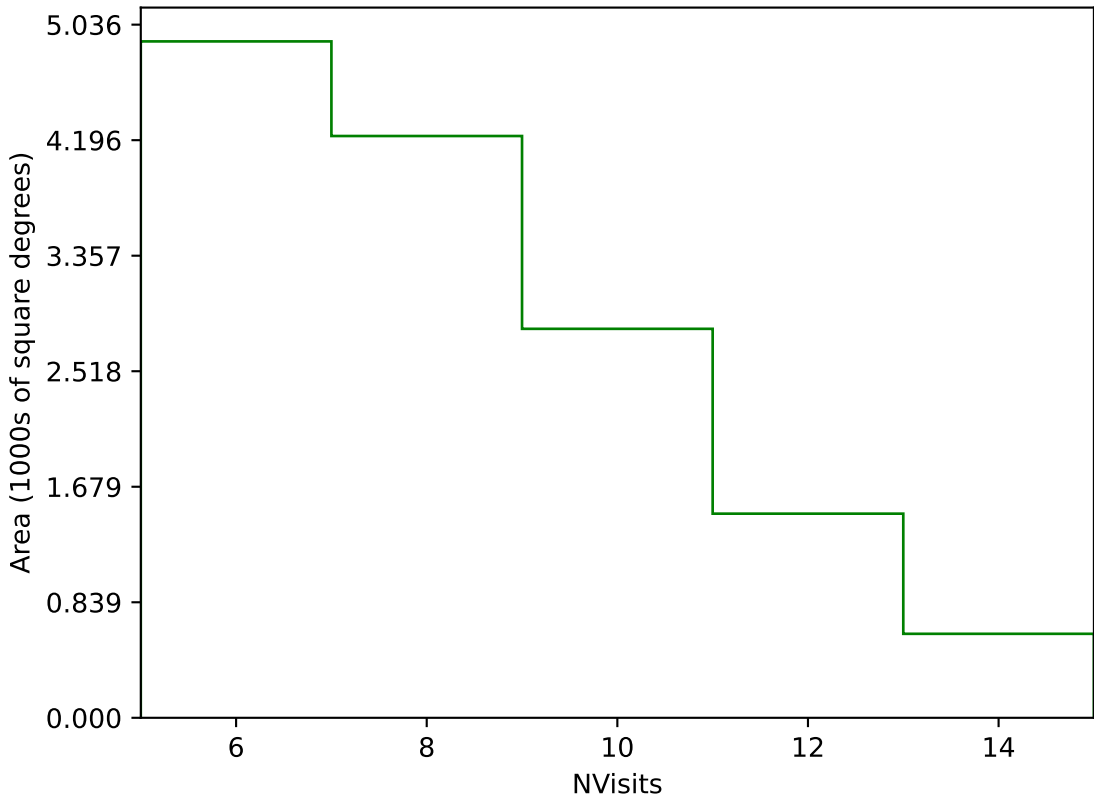
internal_u_expt45_nscale1.1v3.4_10yrs Yr 3-4 g band: NVisits
