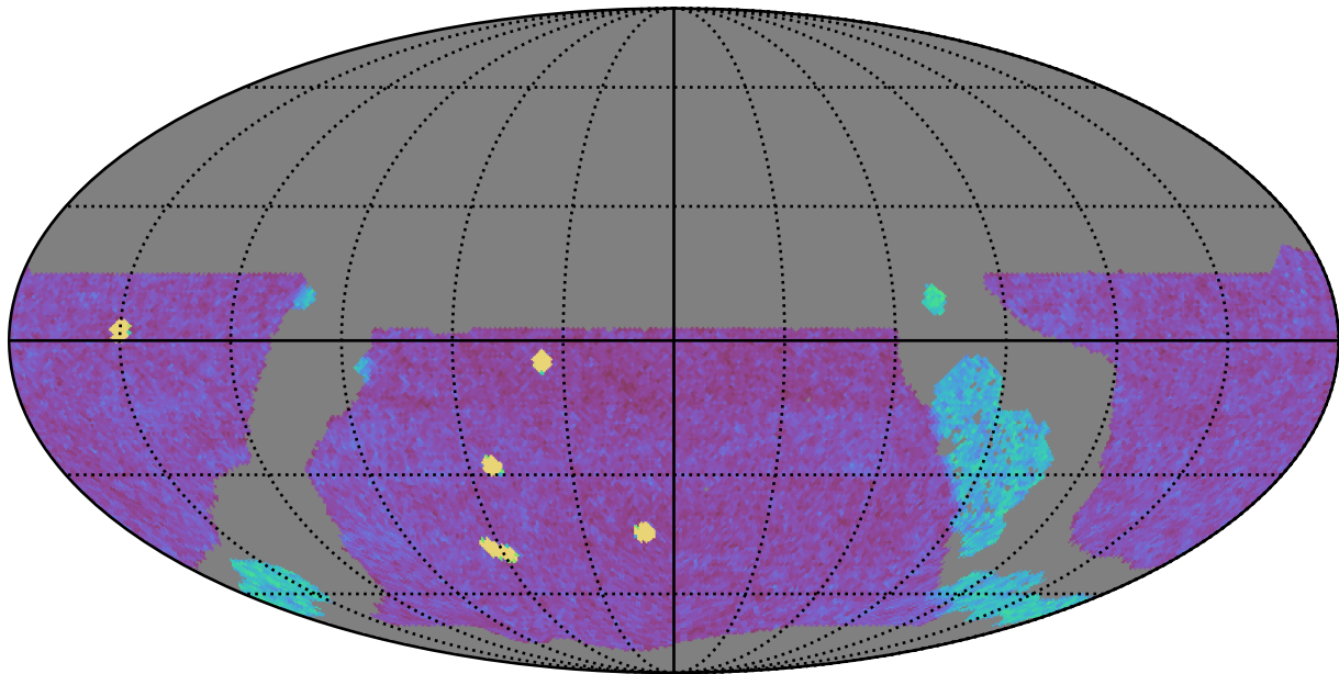
internal_u_expt45_nscale1.1v3.4_10yrs WFD g band: NVisits
