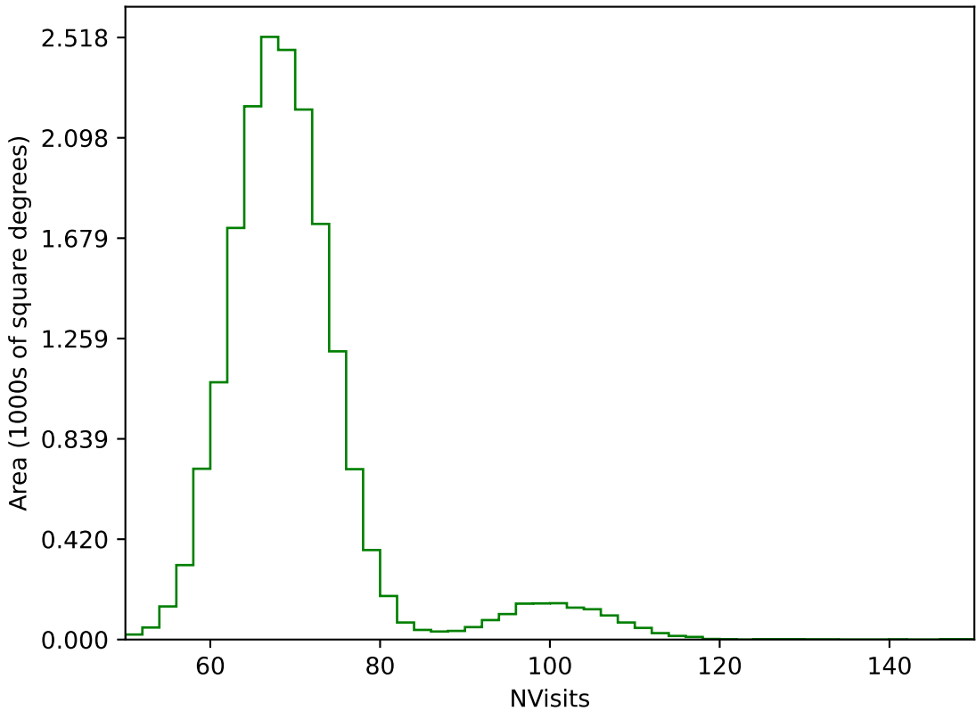
internal_u_expt45_nscale1.1v3.4_10yrs WFD g band: NVisits
