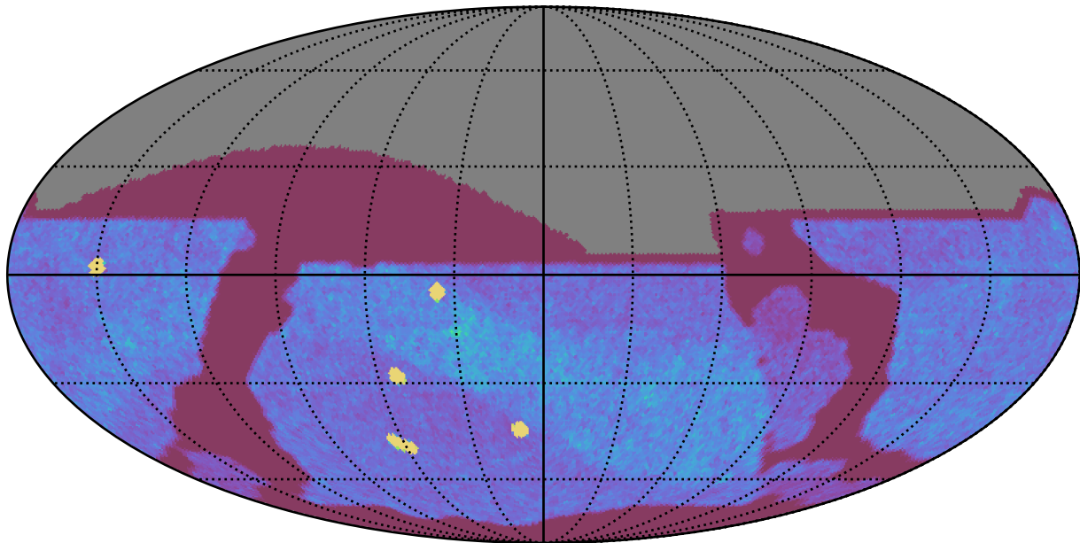
internal_u_expt45_nscale1.1v3.4_10yrs All sky z band: NVisits
