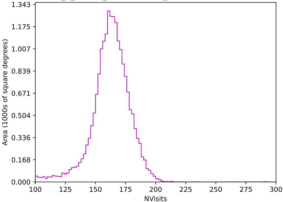
internal_u_expt45_nscale1.1v3.4_10yrs All sky z band: NVisits
