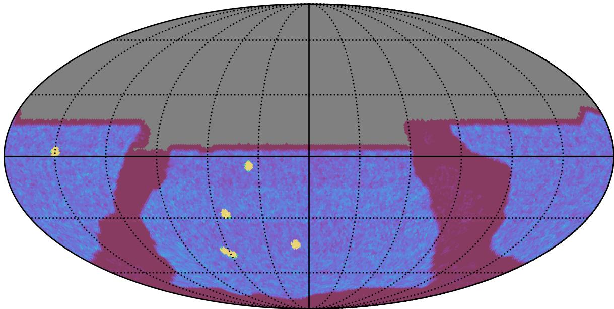
internal_u_expt45_nscale1.1v3.4_10yrs All sky y band: NVisits
