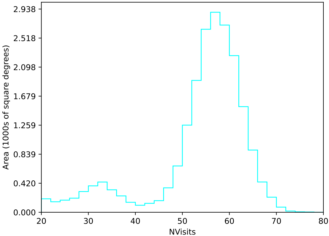
internal_u_expt45_nscale1.1v3.4_10yrs All sky u band: NVisits
