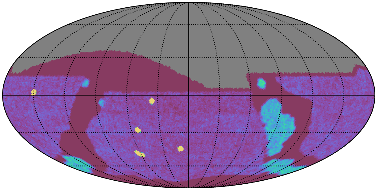
internal_u_expt45_nscale1.1v3.4_10yrs All sky g band: NVisits
