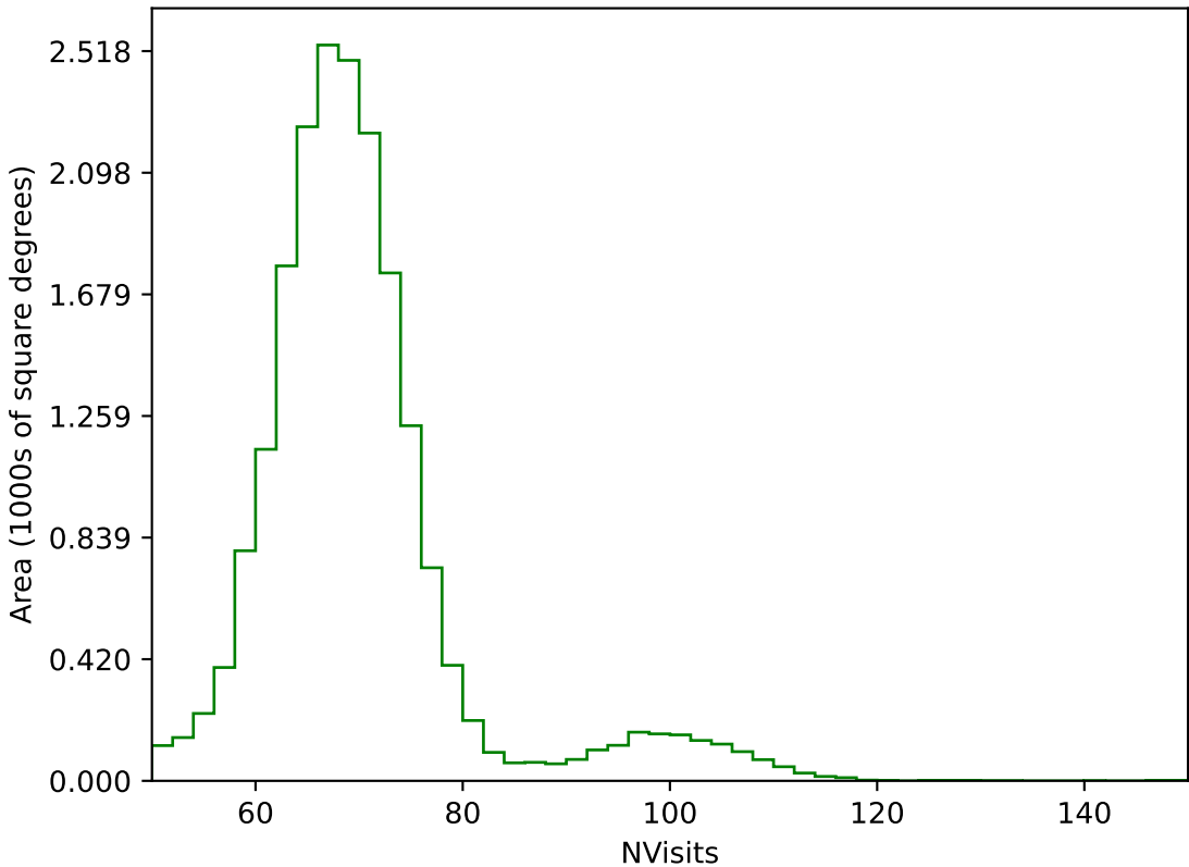
internal_u_expt45_nscale1.1v3.4_10yrs All sky g band: NVisits
